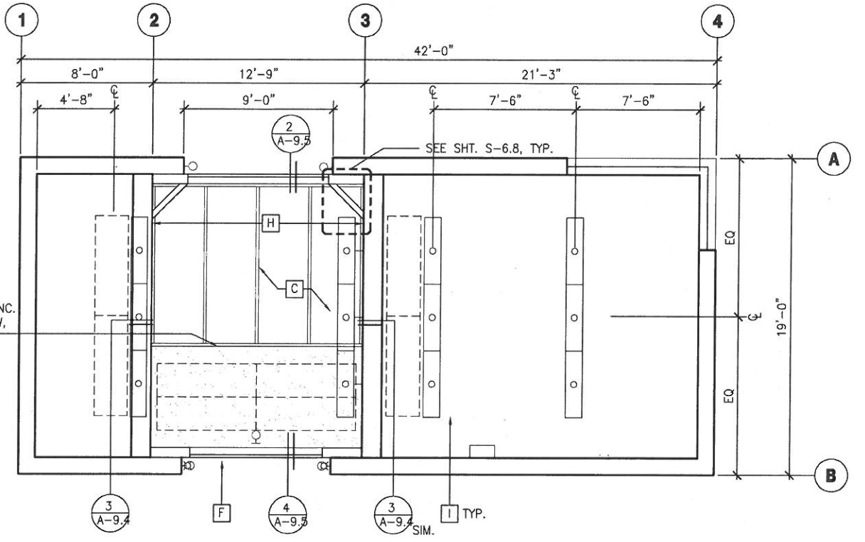
2 REFLECTED CEILING PLAN SCALE: 1/4" = 1'-0"
