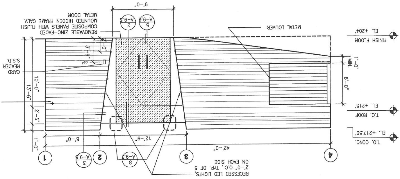
1 NORTH ELEVATION SCALE: 1/4" = 1'-0"
