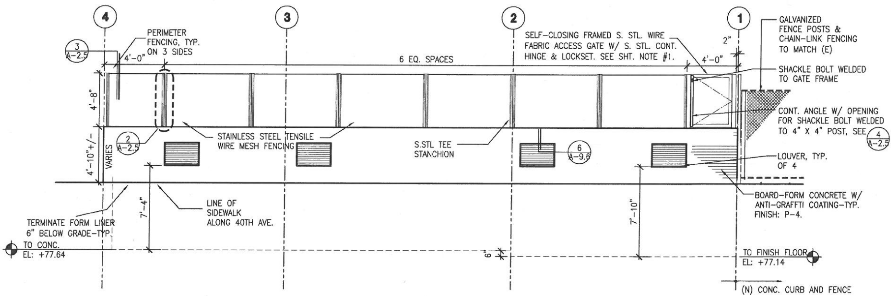
2 EAST ELEVATION - (AT 40TH) SCALE 1/4" = 1'-0"
