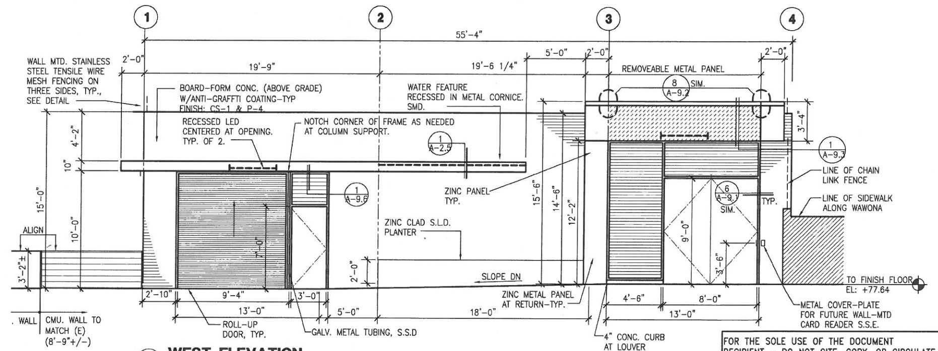
4 WEST ELEVATION SCALE 1/4" = 1'-0"
