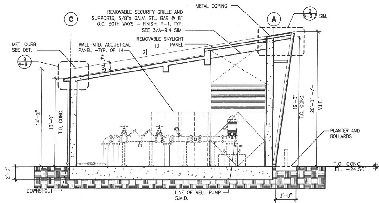
1 BUILDING SECTION - NORTH SCALE: 1/4" = 1'-0"
