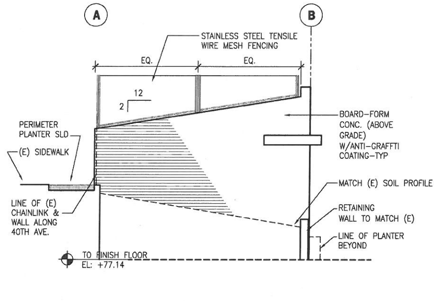
1 NORTH ELEVATION SCALE 1/4" = 1'-0"
