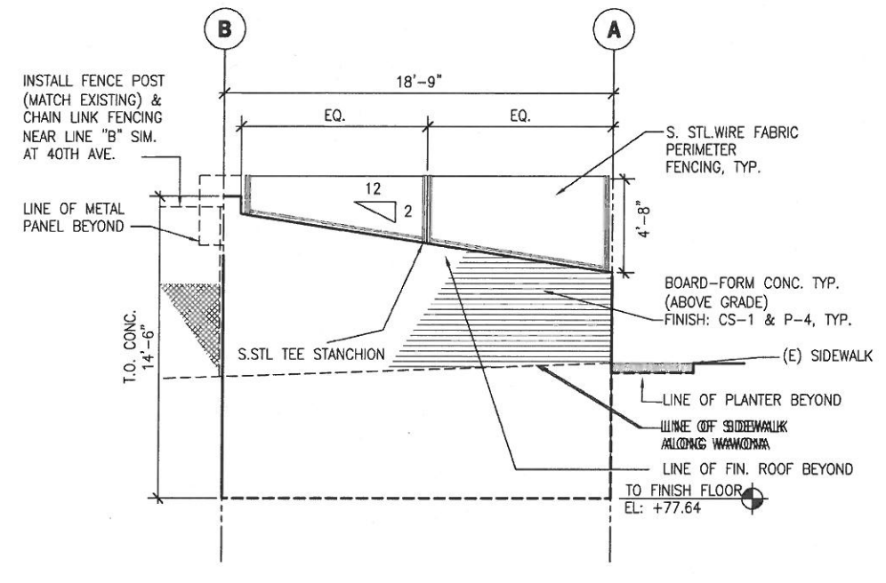
3 SOUTH ELEVATION - (AT WAWONA) SCALE 1/4" = 1'-0"
