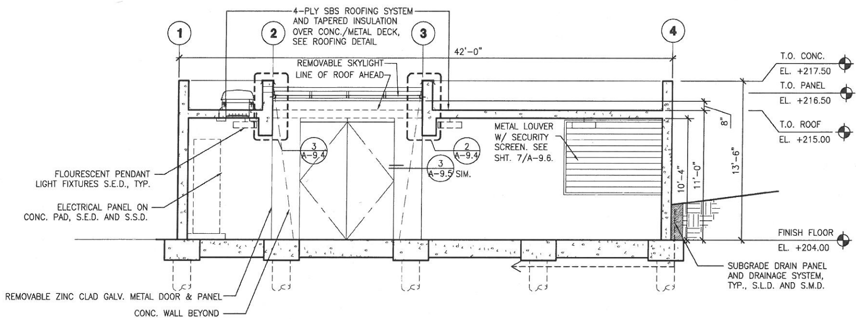
1 BUILDING SECTION - LOOKING NORTH SCALE: 1/4" = 1'-0"
