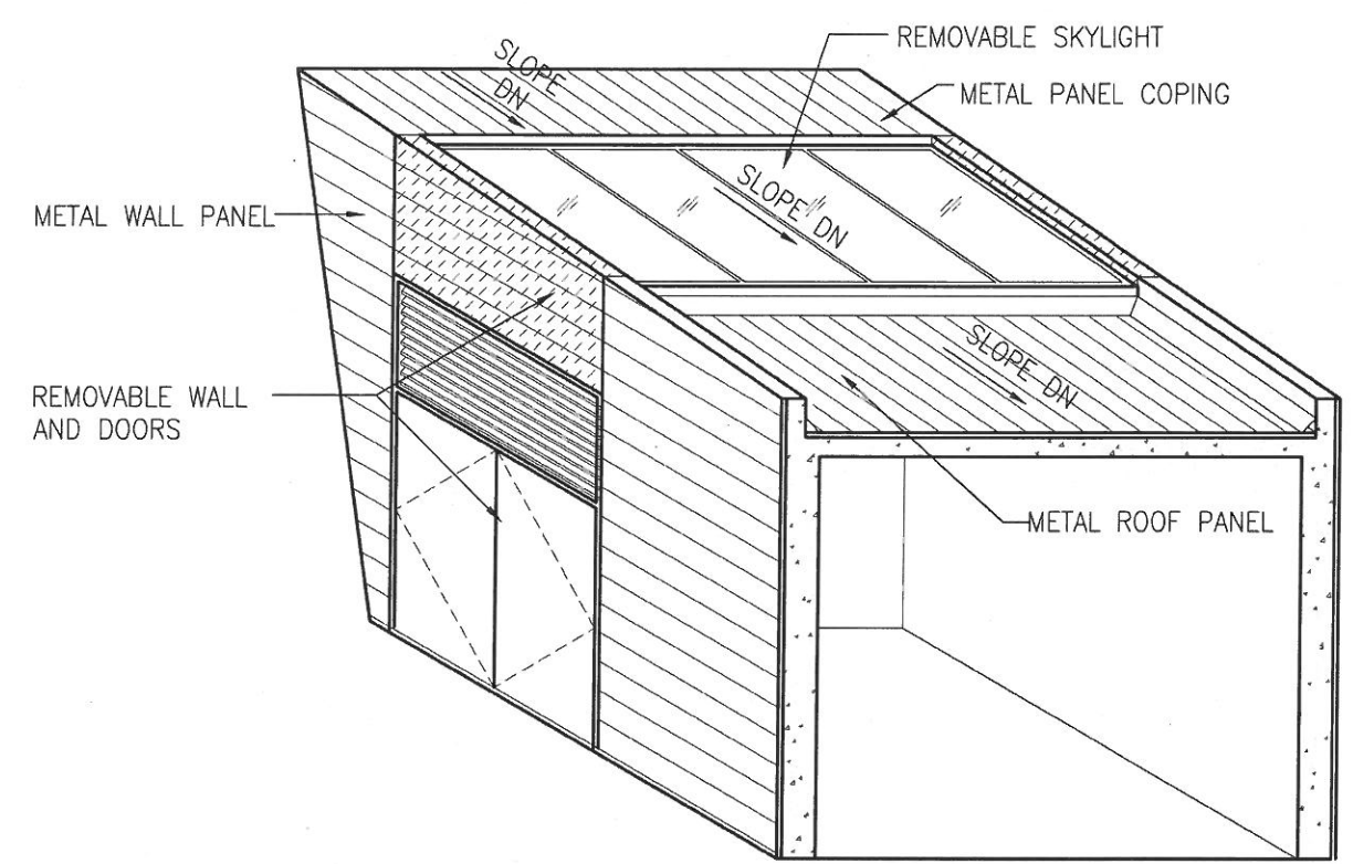
3 PERSPECTIVE VIEW - FOR REFERENCE ONLY SCALE: NTS.
