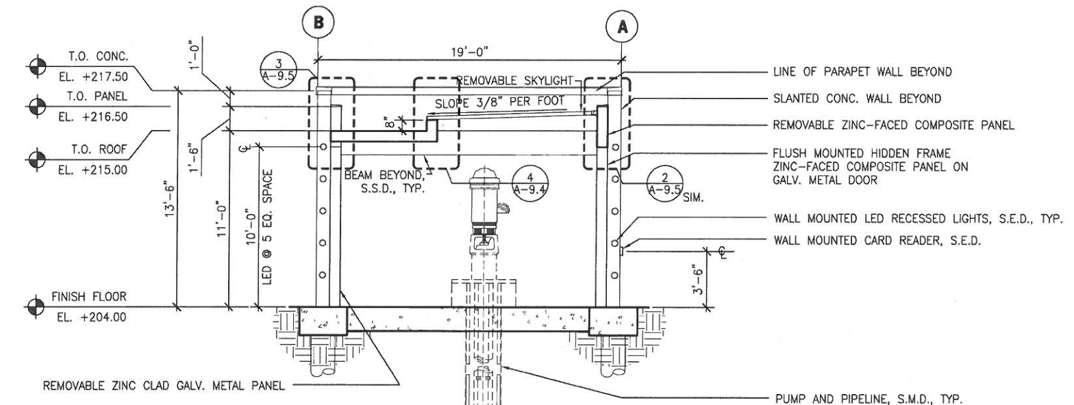
2 BUILDING SECTION - LOOKING WEST SCALE: 1/4" = 1'-0"
