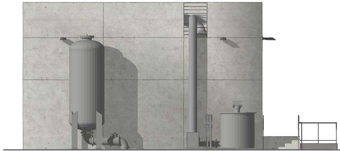
EAST ELEVATION
