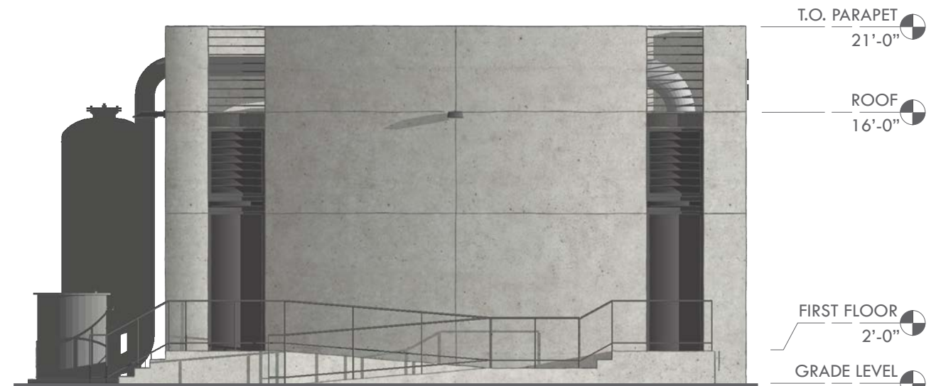
NORTH ELEVATION
