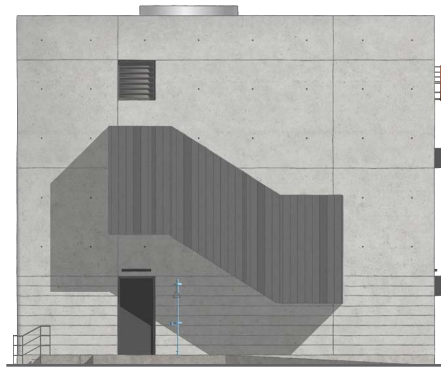
WEST ELEVATION
