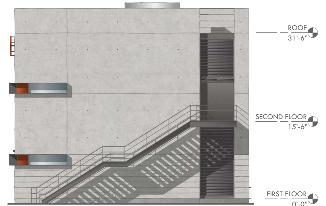
EAST ELEVATION
