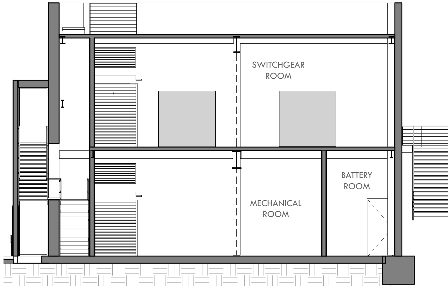
SECTION B-B
