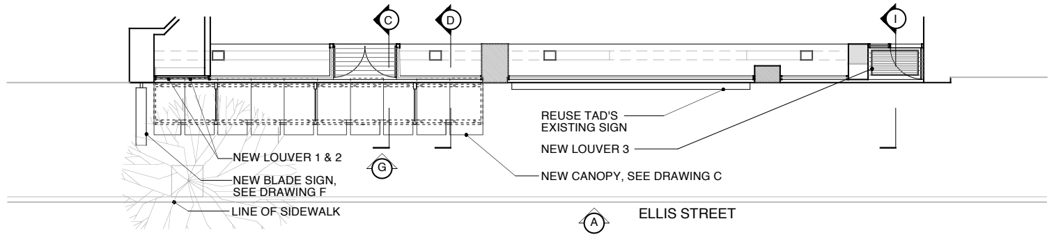
B. REFLECTED CEILING PLAN AT STOREFRONT
