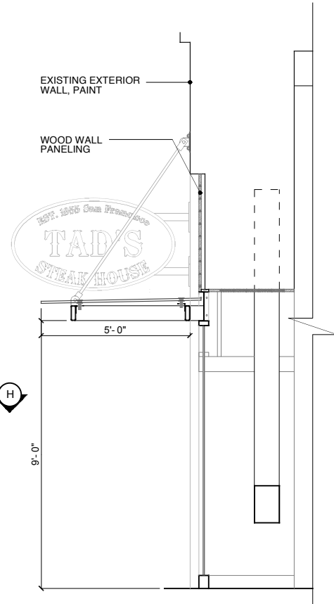
D. ENLARGED PARTIAL SECTION
