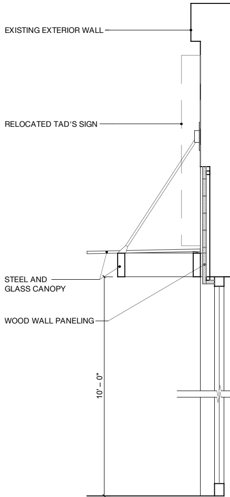
B. ENLARGED PARTIAL SECTION
