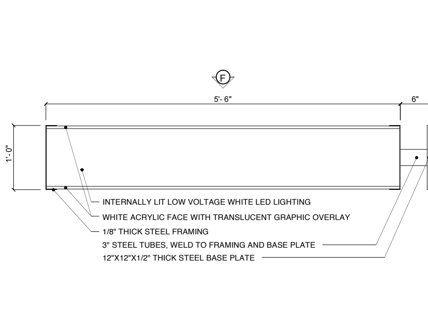
E. SECTION DETAIL - BLADE SIGN
