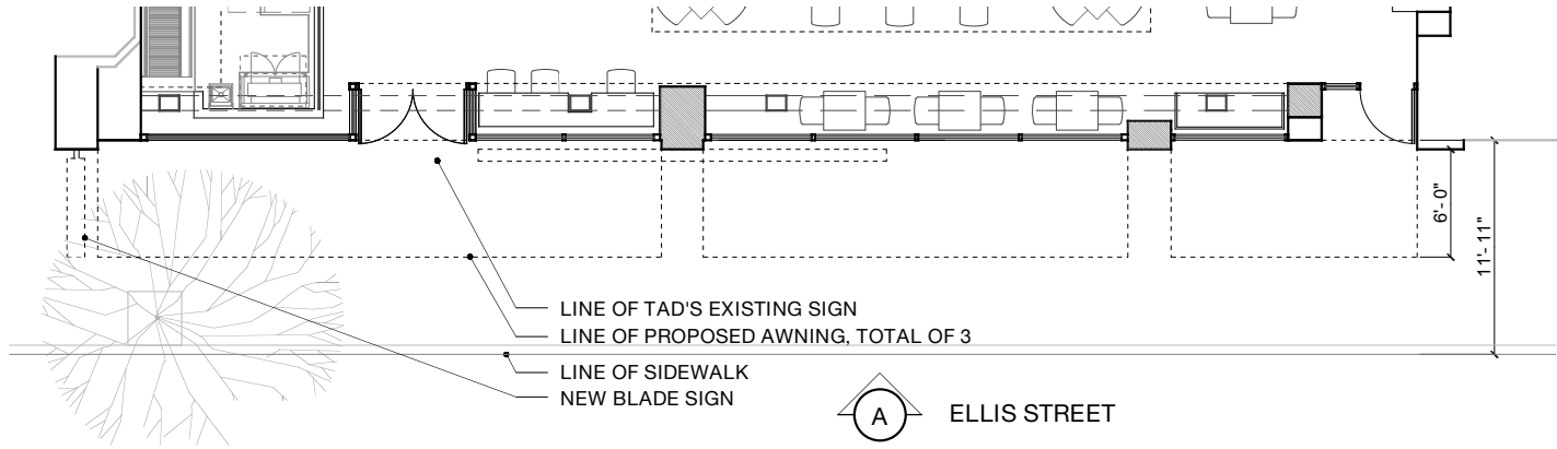
C. PARTIAL PLAN AT STOREFRONT
