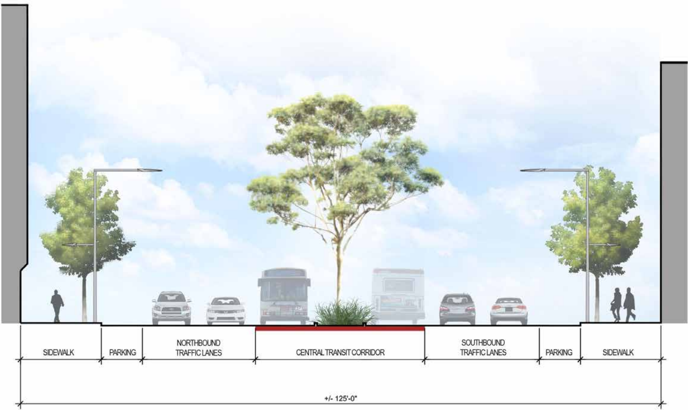
VAN NESS BRT SECTION A: NO PLATFORM
