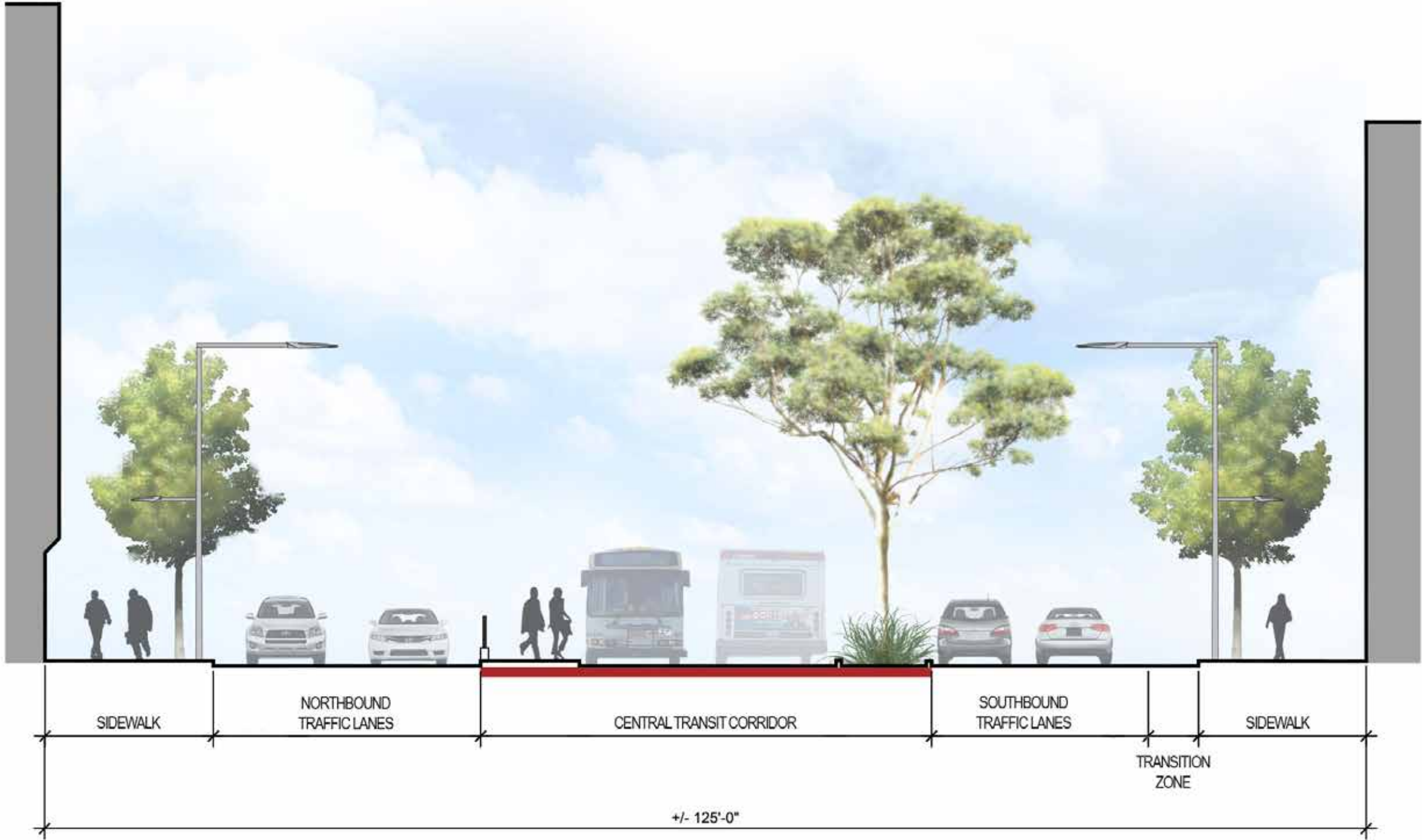
VAN NESS BRT SECTION D: DOUBLE PLATFORM WITH PLANTING
