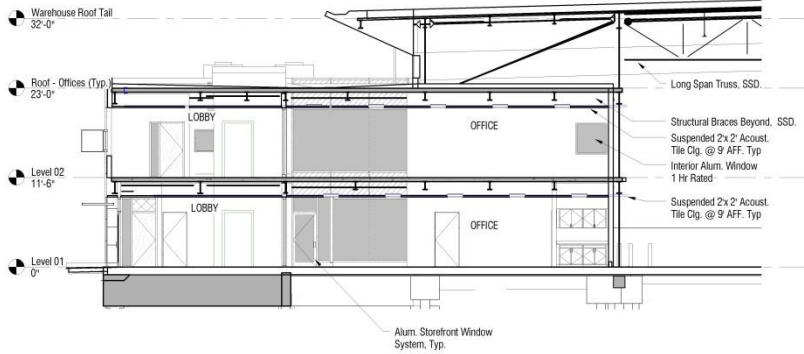
Partial Section @ Pod
