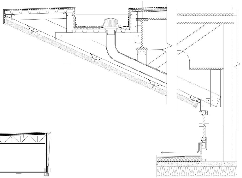
Soffit/Clerestory Detail
