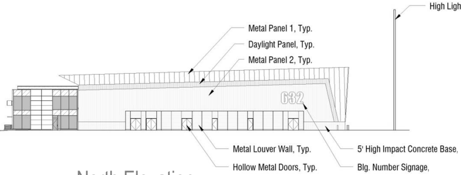
North Elevation
