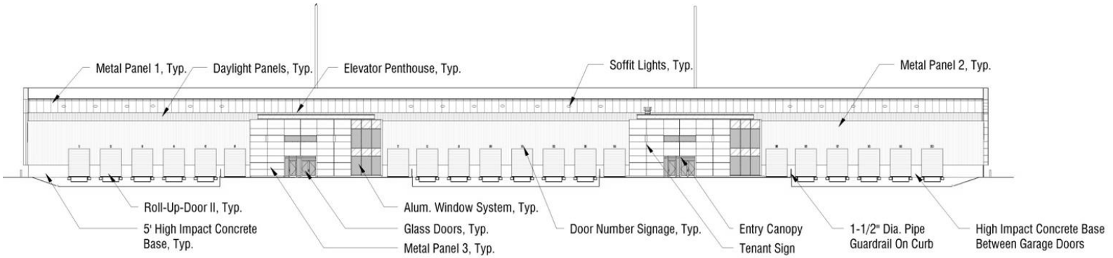
East Elevation
