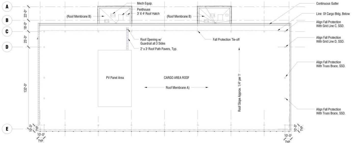
Roof Level
