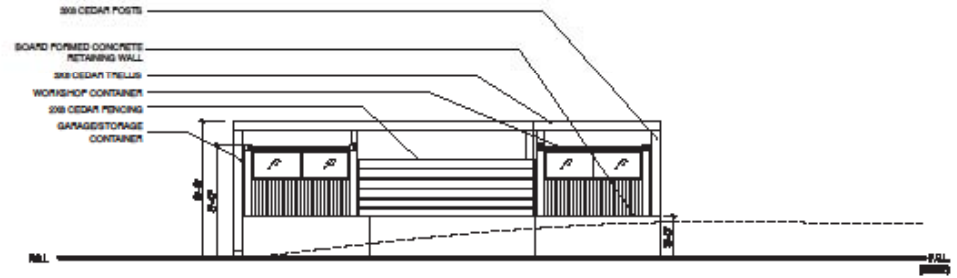
EAST ELEVATION
