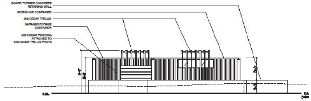
NORTH ELEVATION
