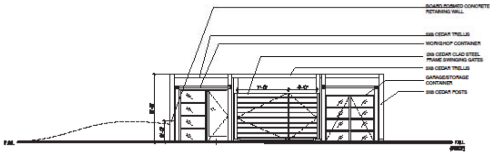
WEST ELEVATION
