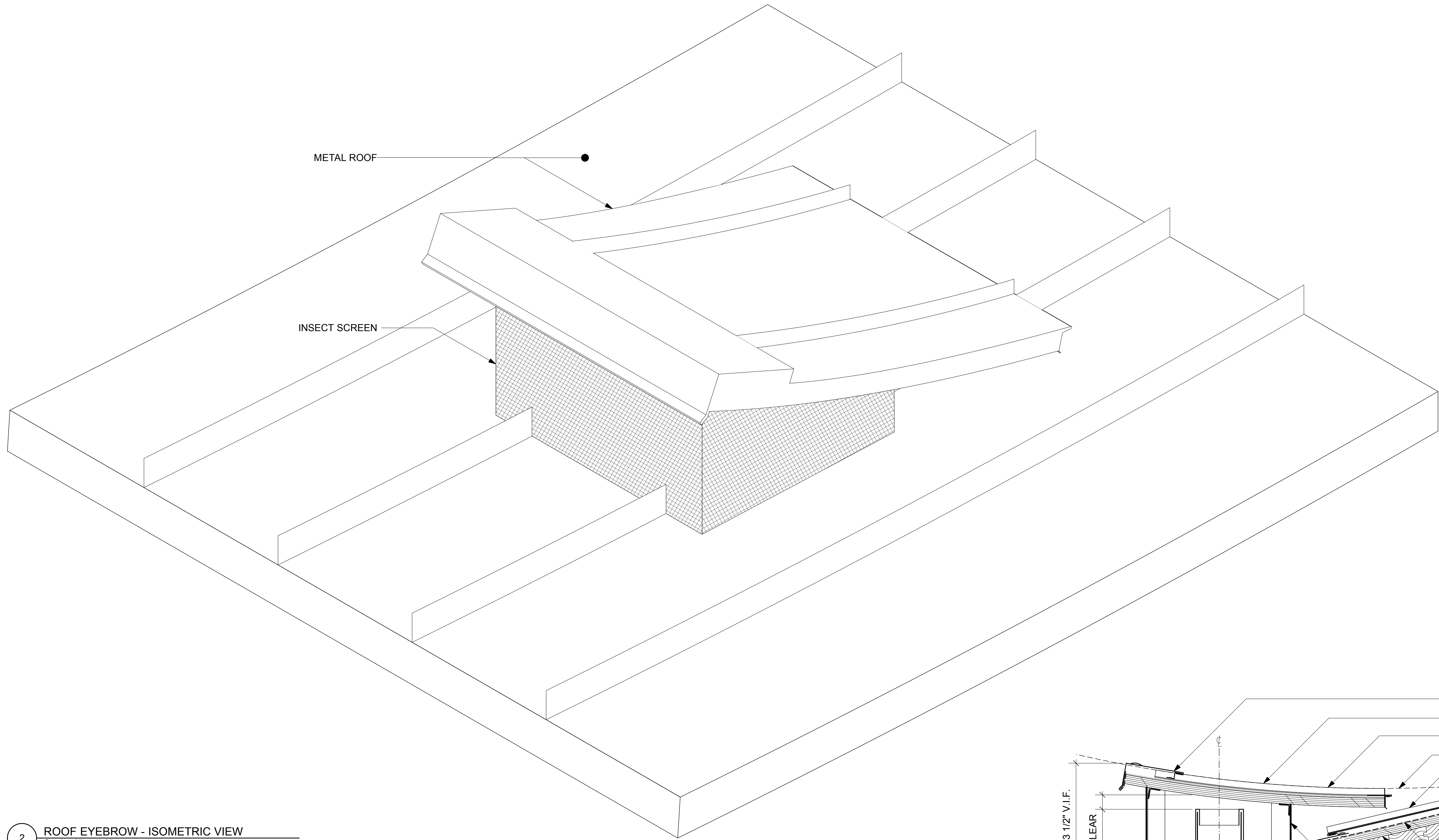
2 ROOF EYEBROW - ISOMETRIC VIEW Scale: 3" = 1'-0"
