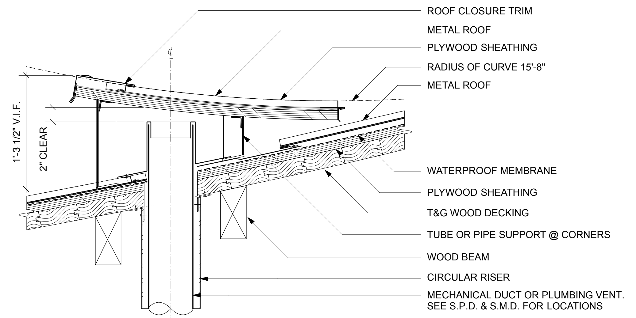
1 ROOF EYEBROW DETAIL Scale: 1 1/2" = 1'-0"
