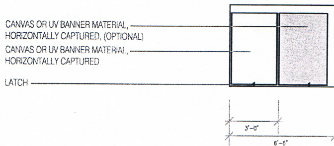
TOP VIEW (WITH SUNSHADES CLOSED)
