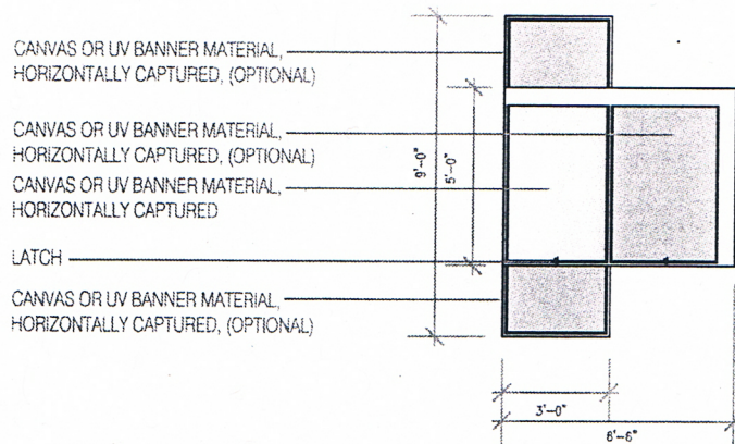
TOP VIEW (WITH SUNSHADES OPEN)
