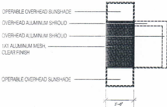
PLAN @ TABLE TOP HEIGHT, (+2'-6" ABOVE FLOOR)
