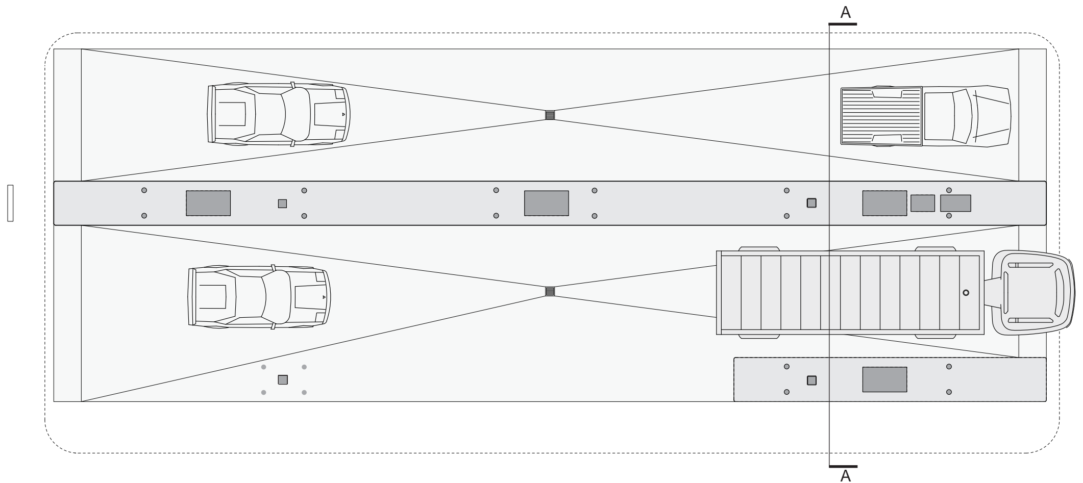
Fueling Station Plan
