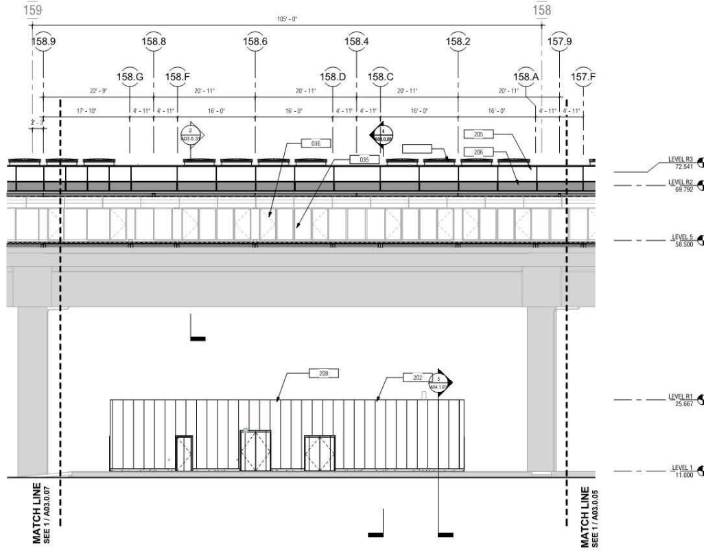
1 EXTERIOR ELEVATION - WEST SECTOR 2 OF 3 A03.0.01 | A03.0.06 SCALE: 1/8" = 1'-0"
