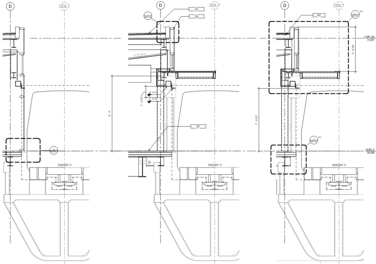
3 CURTAINWALL SECTION - SOUTH OF BARRIER WALL A03.0.02 A03.0.31 SCALE: 1/2" = 1'-0"
