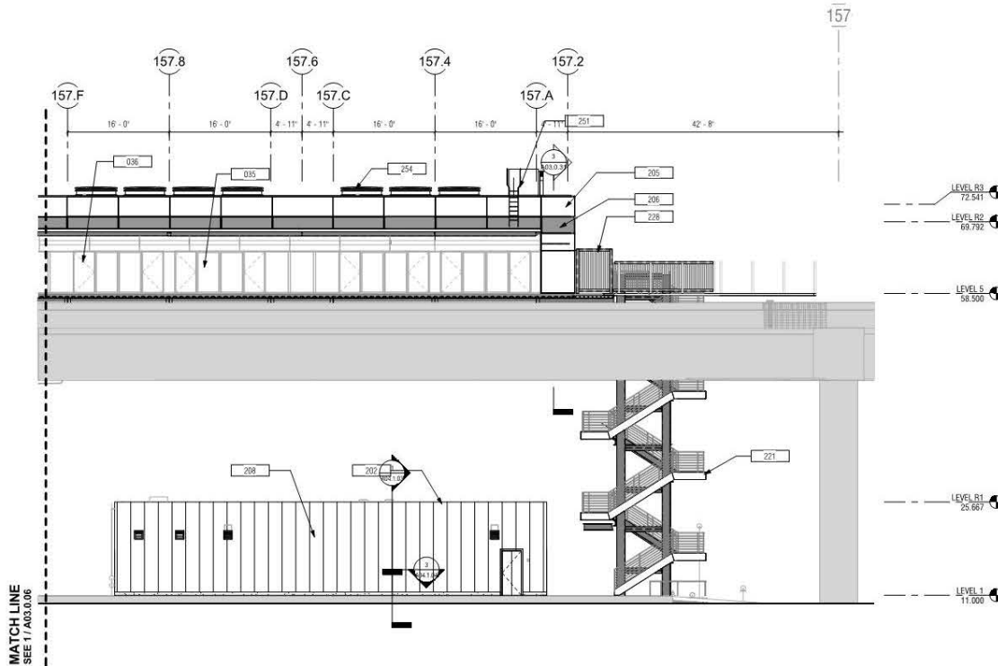
1 EXTERIOR ELEVATION - WEST SECTOR 1 OF 3 A03.0.01 A03.0.05 SCALE: 1/8" = 1'-0"
