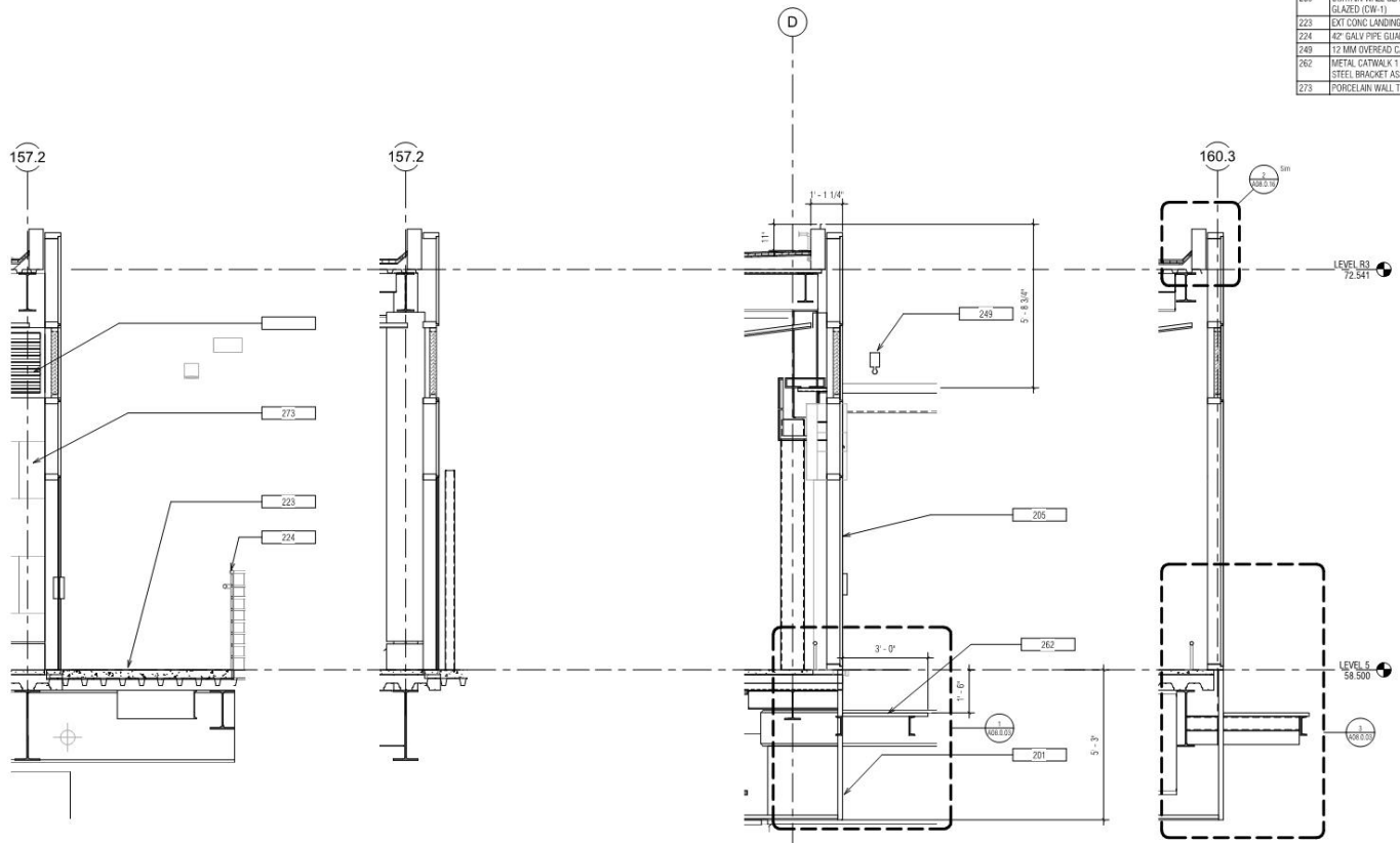
4 CURTAINWALL SECTION - DOOR PANEL SCALE: 1/2" = 1'-0" 3 CURTAINWALL SECTION - SOUTH END WALL TYP SCALE: 1/2" = 1'-0" 2 CURTAINWALL SECTION - LONGITUDINAL WALL TYP SCALE: 1/2" = 1'-0" 1 CURTAINWALL SECTION - NORTH ENDWALL SCALE: 1/2" = 1'-0"
