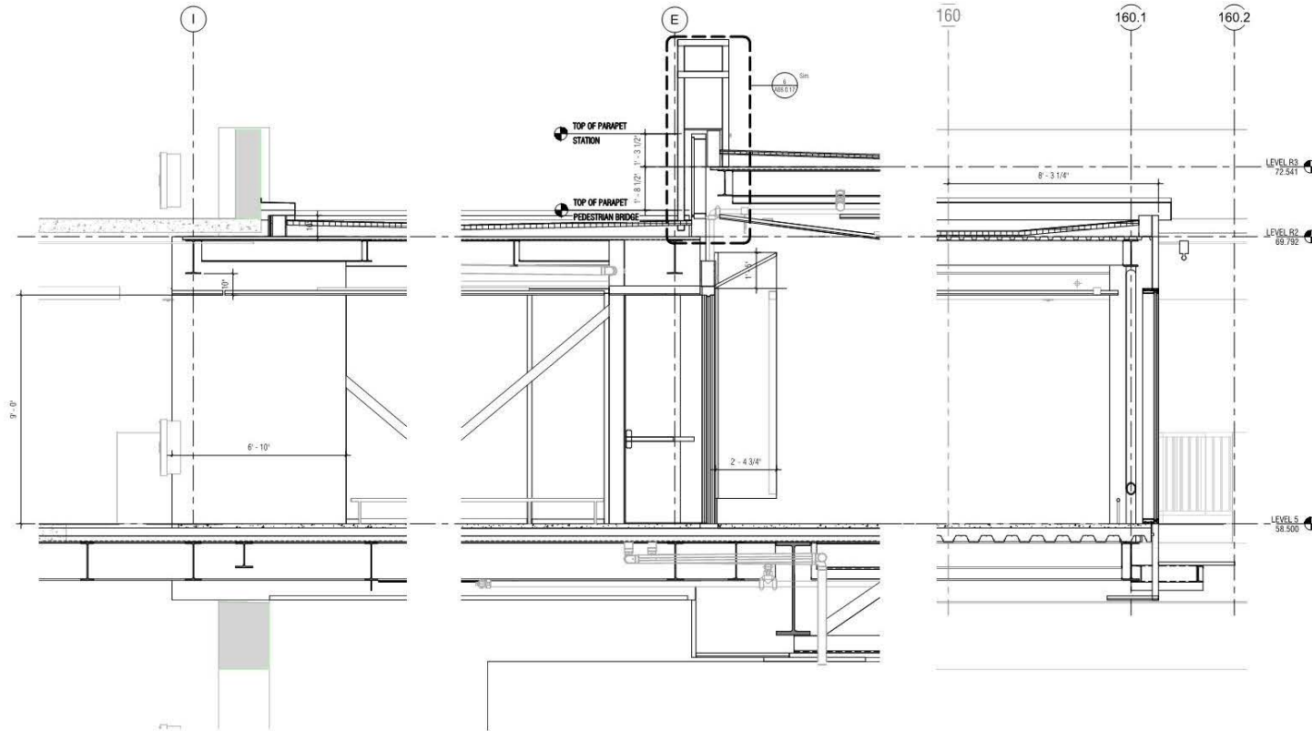
3 CONNECTOR BRIDGE AT GARAGE A05.5.03 A03.0.33 SCALE: 1/2" = 1'-0"
