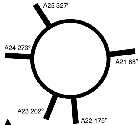
SECTION DIAGRAM 1/4" = 1"
