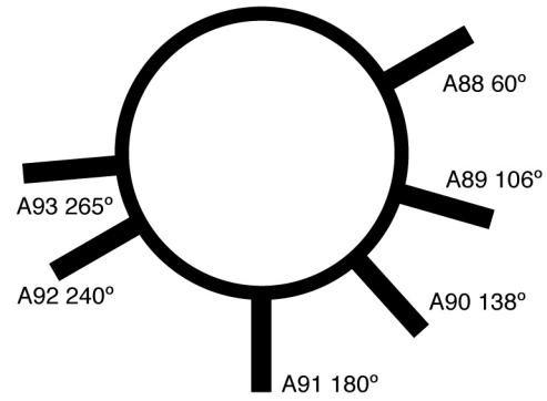
▲ N 0°/360° SECTION DIAGRAM 1/4" = 1"
