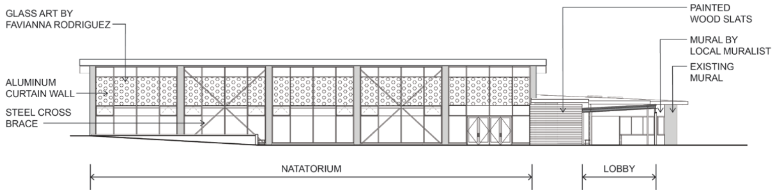
WEST ELEVATION NATATORIUM
