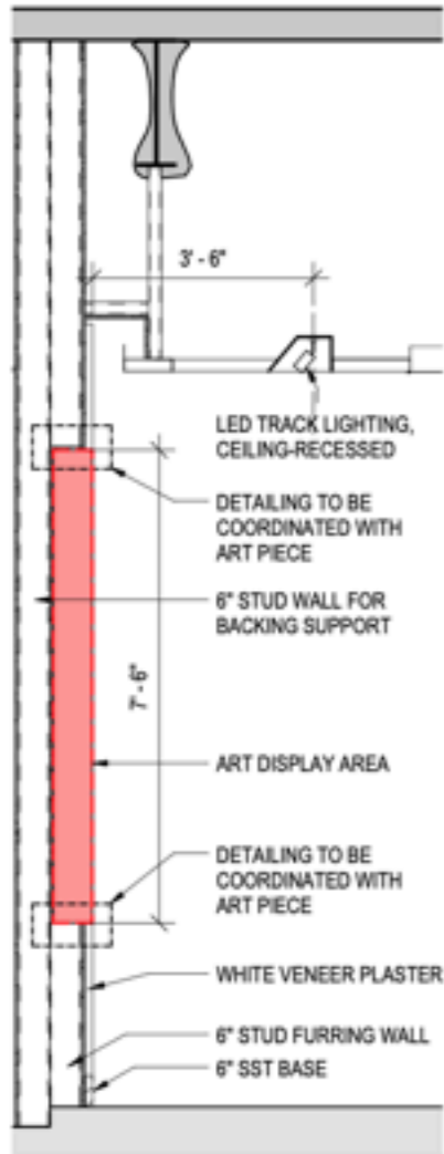
A-A Typical Section at Art Wall Scale: 3/4" = 1'-0"
