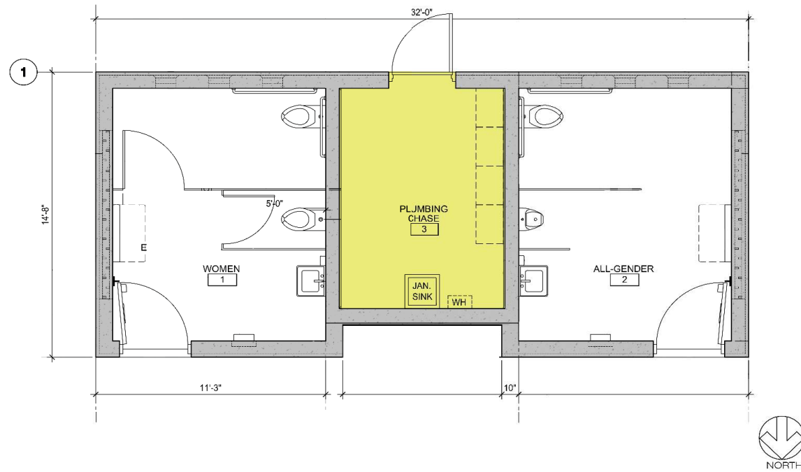
PROTOTYPE PLAN APPROVED BY CDR IN APRIL 2016
