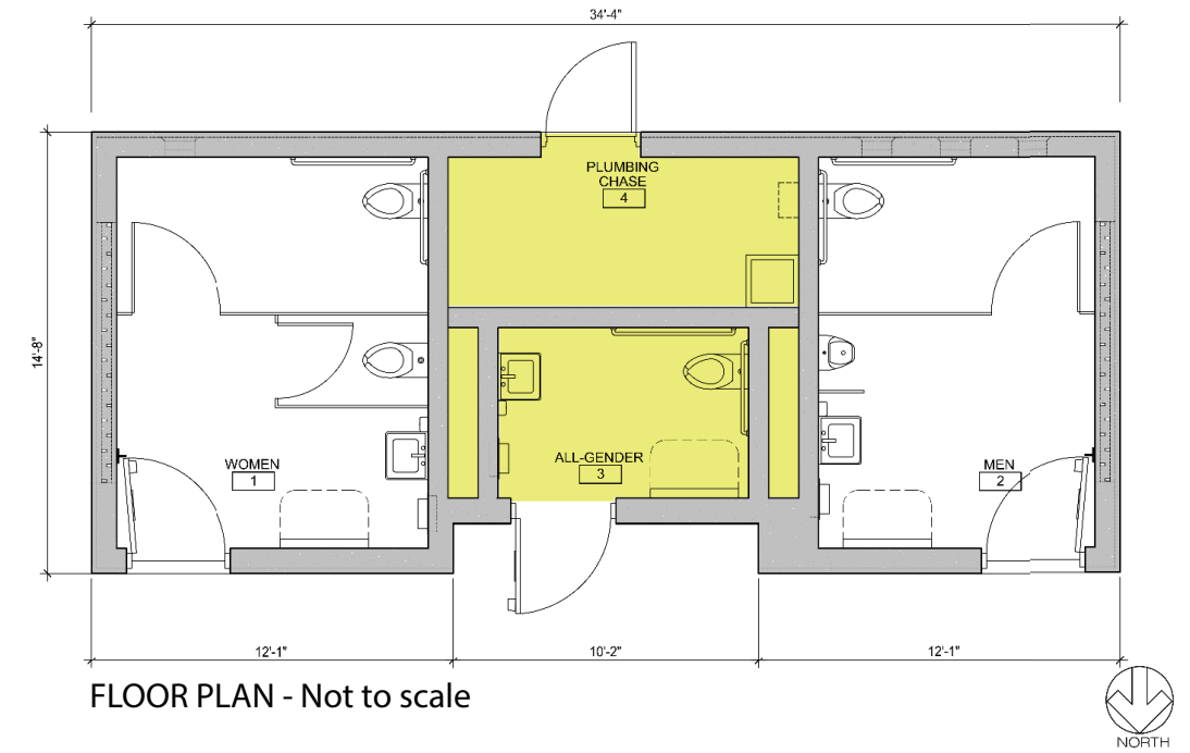
MODIFIED PLAN INCORPORATING ALL GENDER RESTROOM
