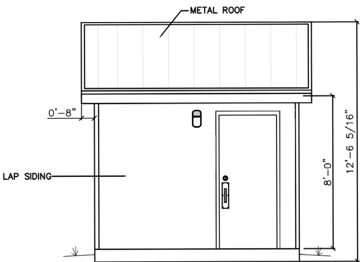
REAR ELEVATION
