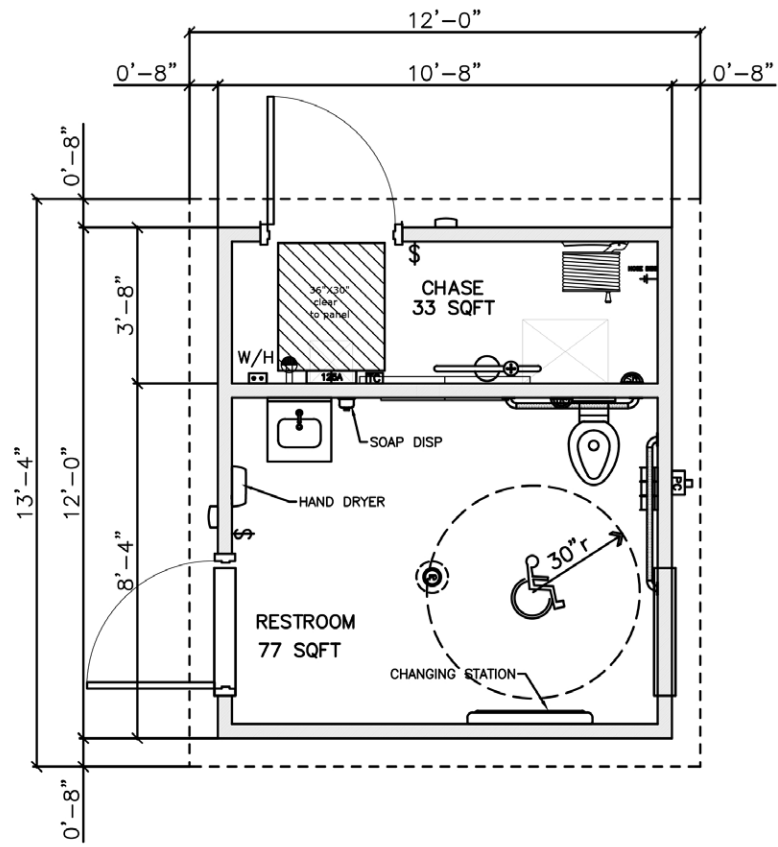
FLOOR PLAN 128 SQFT
