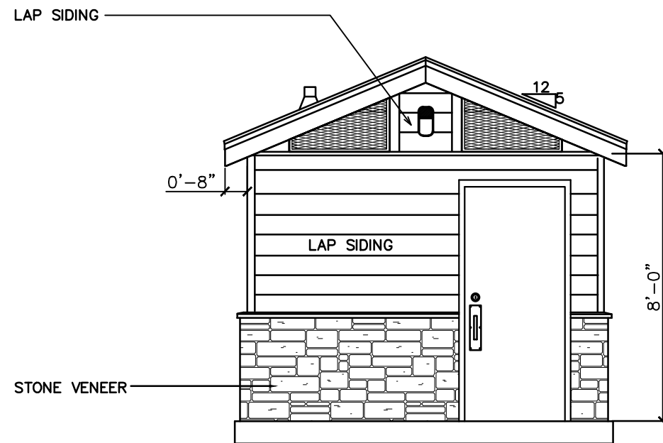
REAR ELEVATION
