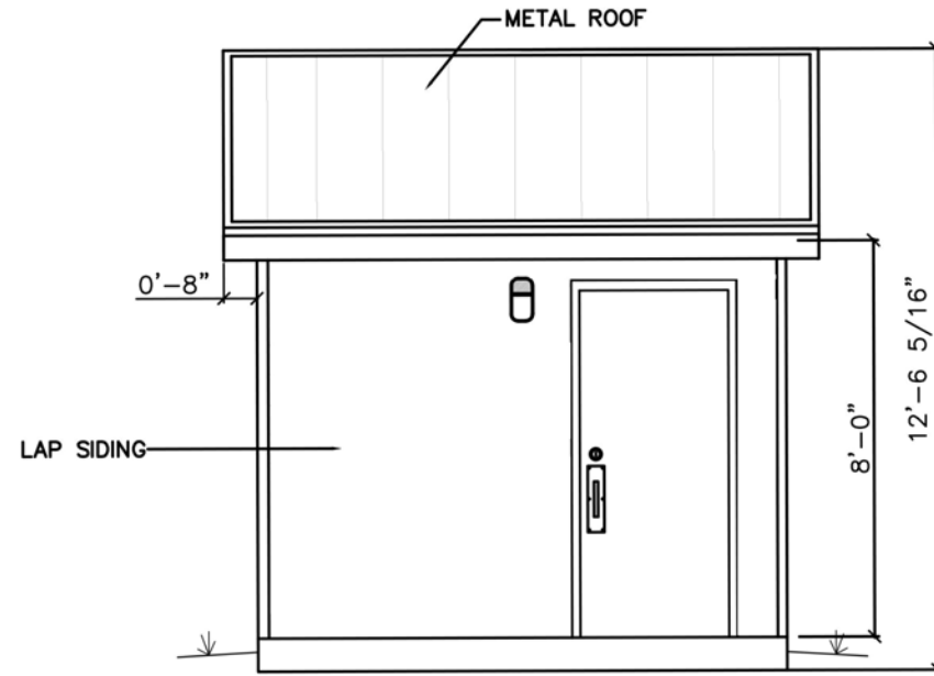
Front Elevation (East)
