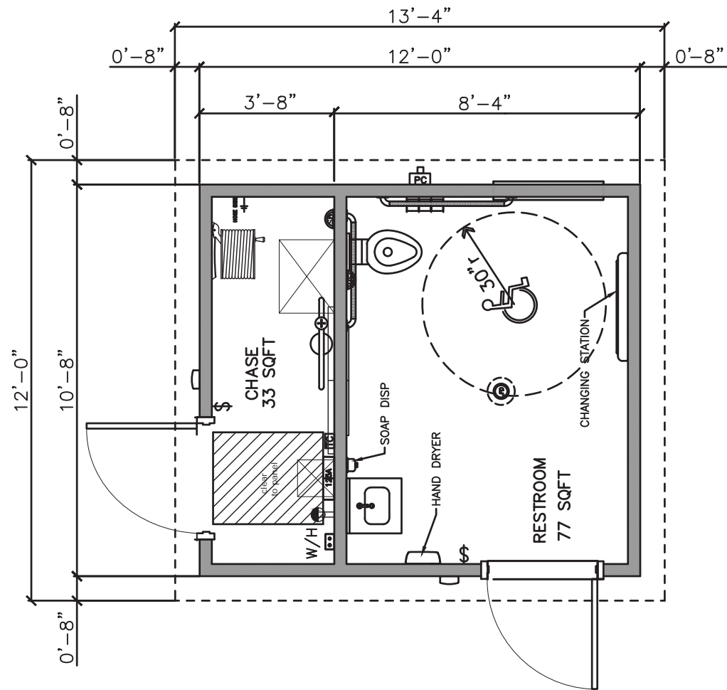
Floor Plan (128 SQFT)
