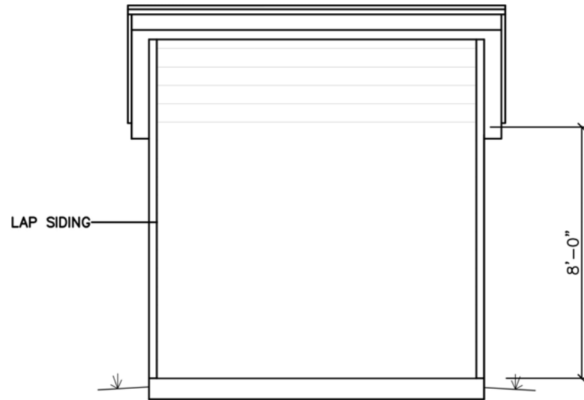
Back Elevation (West)
