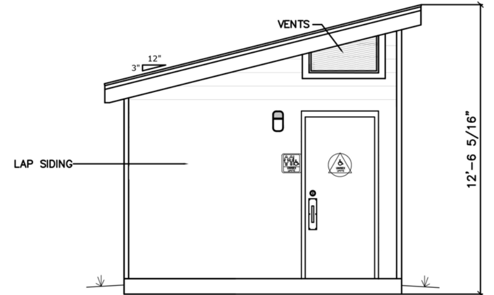
Right Elevation (North)
