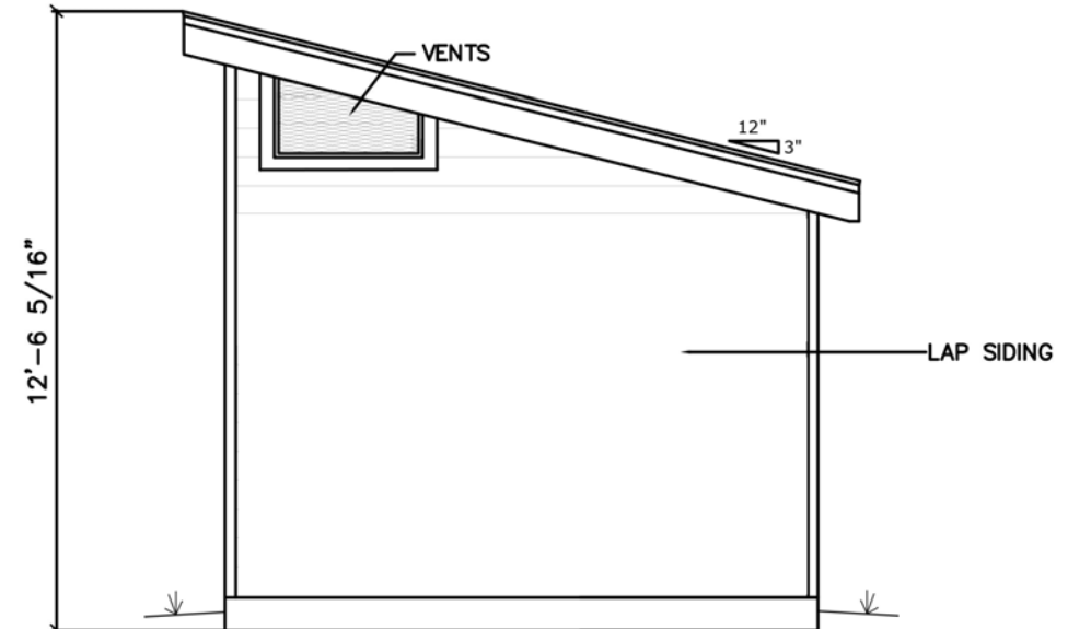
Left Elevation (South)
