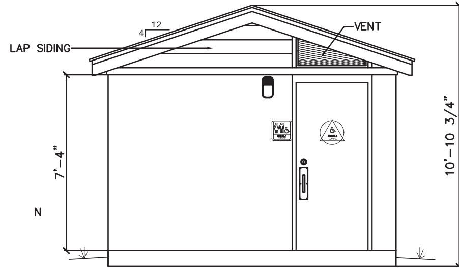
Front Elevation (East)
