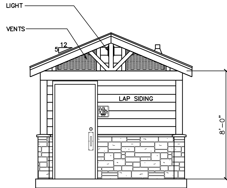
FRONT ELEVATION
