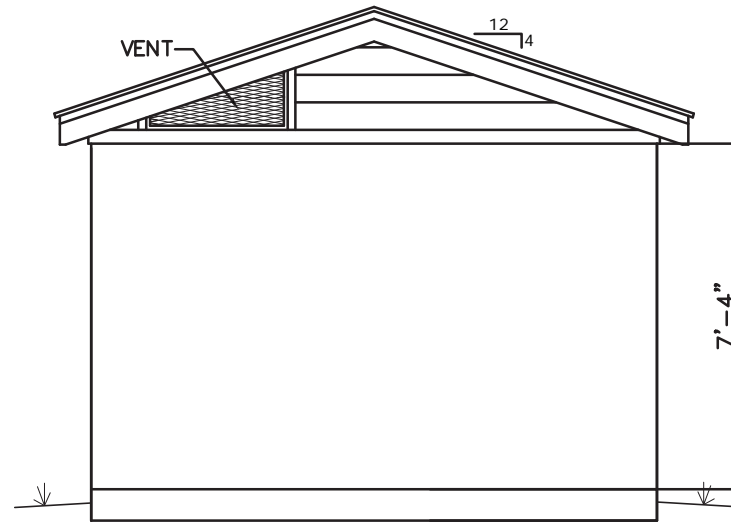
Back Elevation (West)
