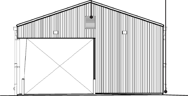
SOUTH ELEVATION
