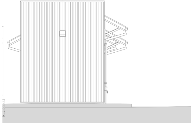
NORTH ELEVATION
