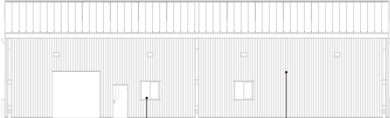
EAST ELEVATION
