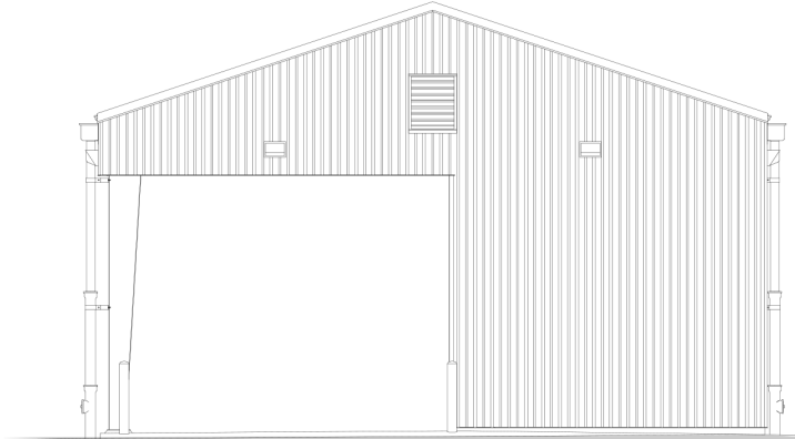
SOUTH ELEVATION
