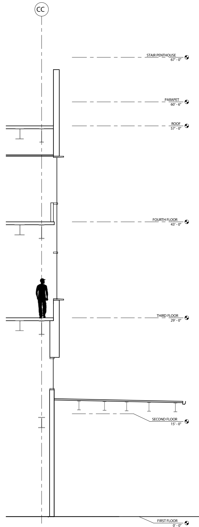
2 South Facade Section 1/8" = 1'-0"
