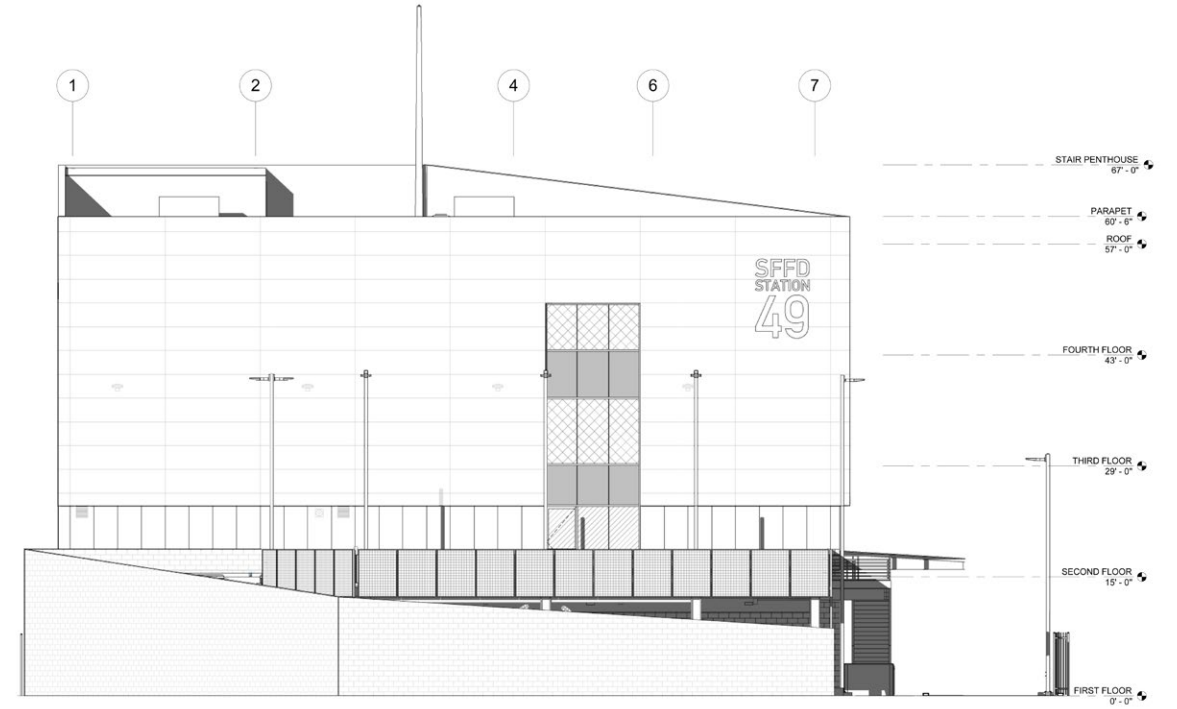
4 Phase 3 - South Elevation w/Parking Structure
