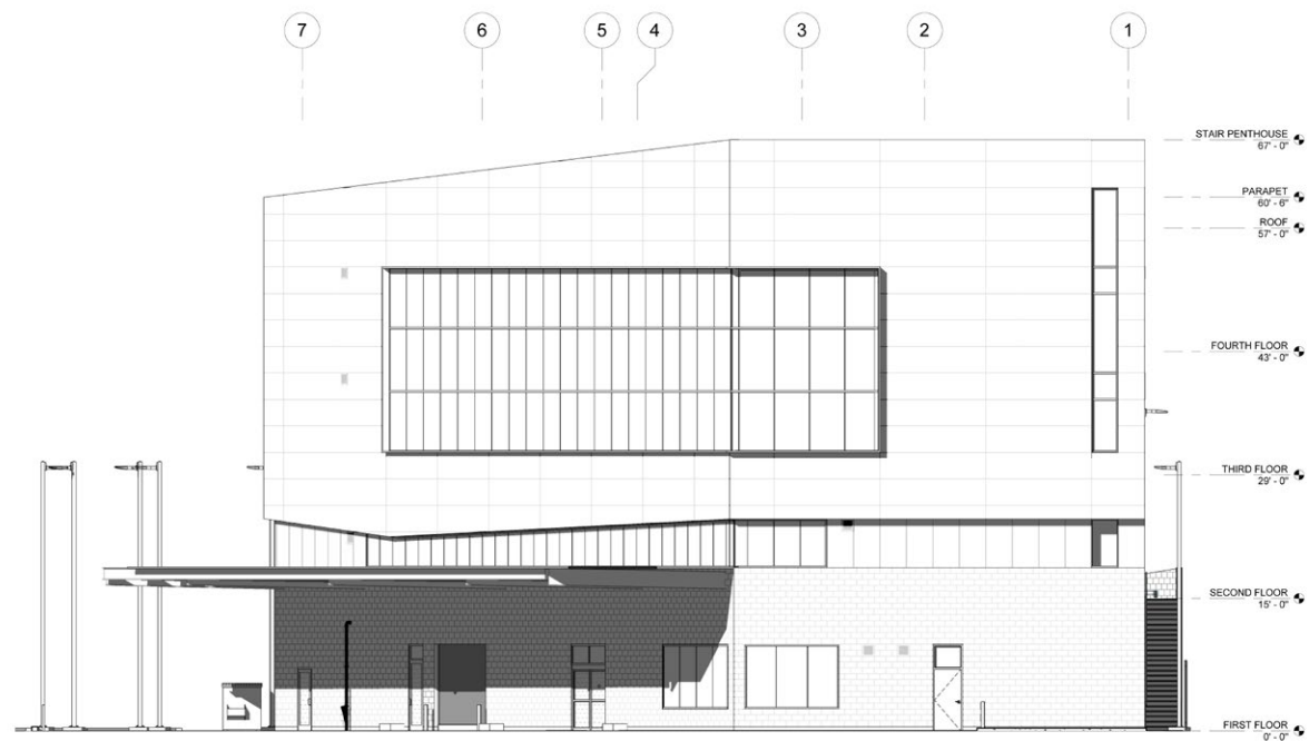
Phase 2 - North Elevation
