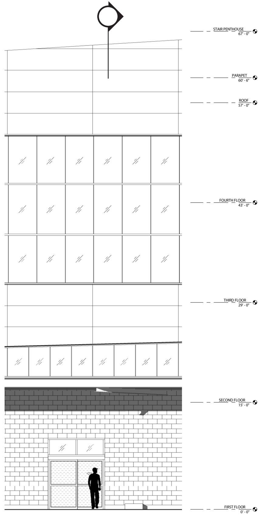
1 South Elevation - Partial 1/8" = 1'-0"
