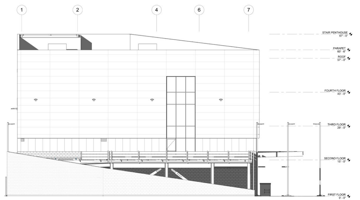
Phase 2 - South Elevation w/Parking Structure
