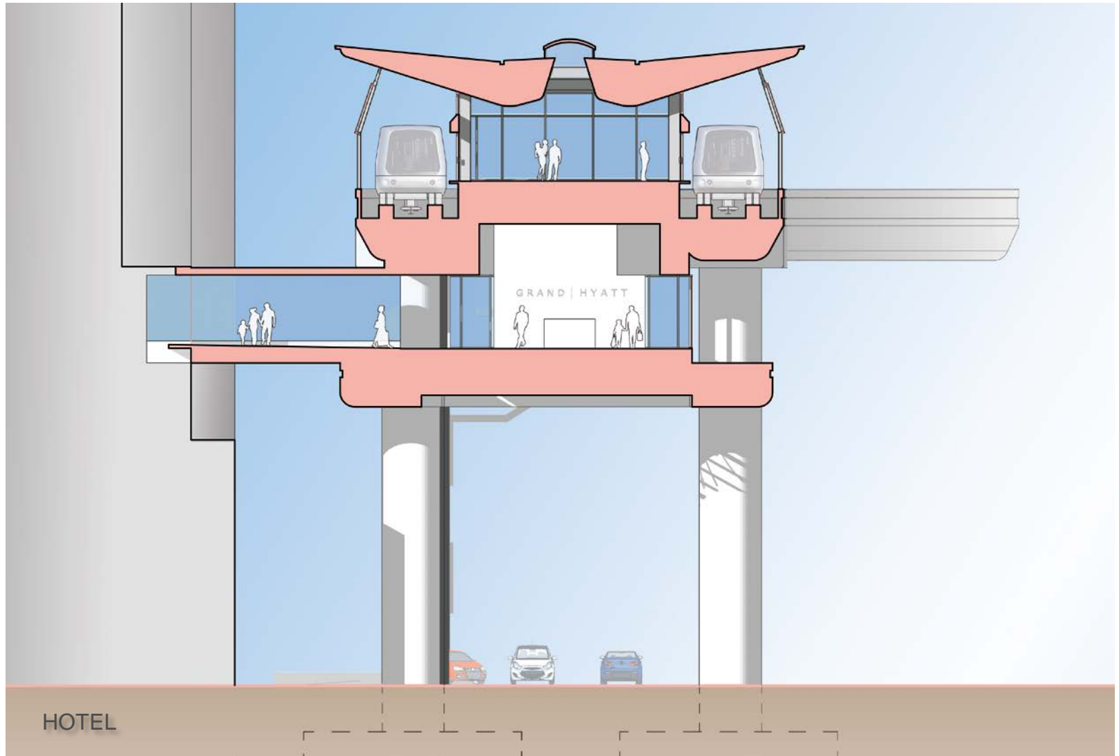
Hotel Station – Transverse Section
