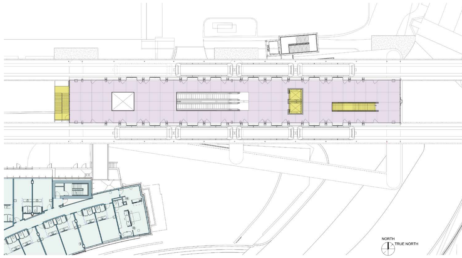
Hotel Station – Overall Platform Plan
