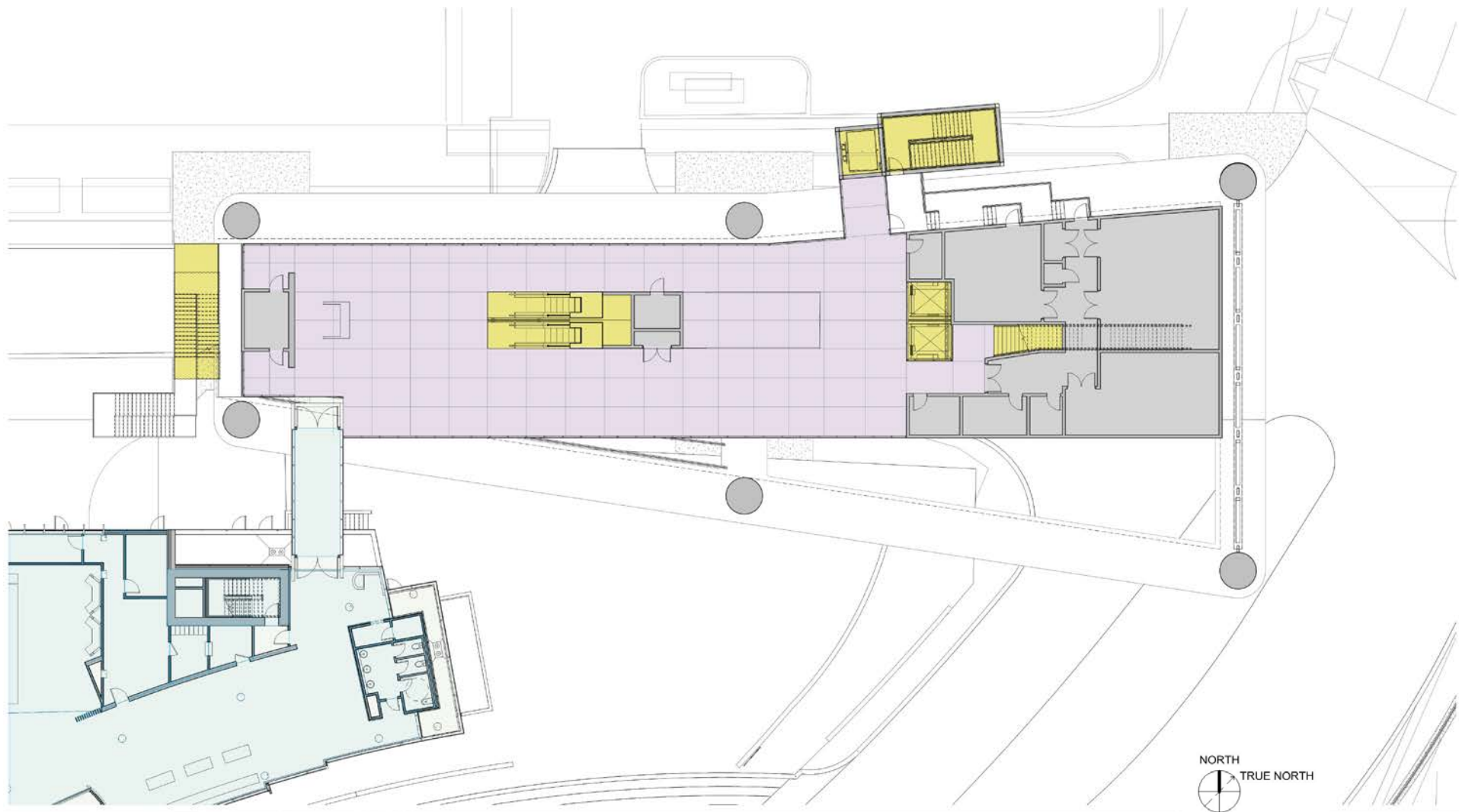
Hotel Station – Overall Concourse Plan
