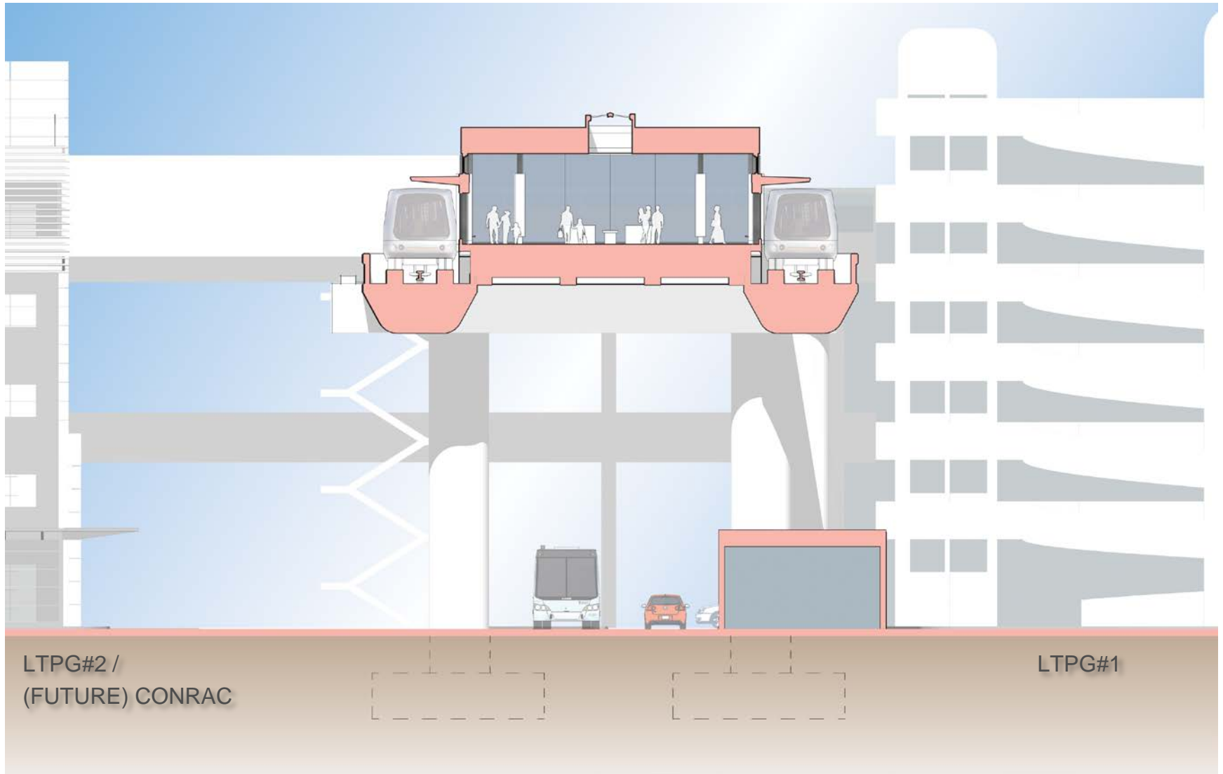
LTP Station – Transverse Section
