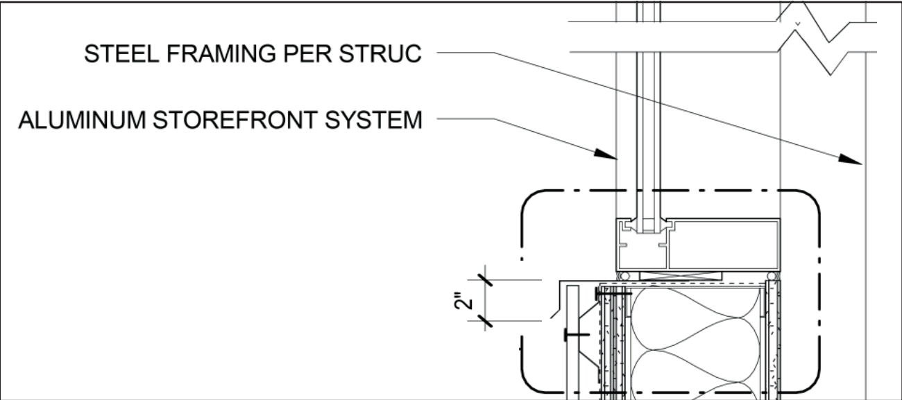
Enlarged Detail C at Exterior Window Sill nts
