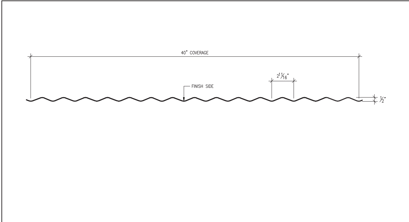
Profile Section of Formed Metal Panel - Pattern B nts
