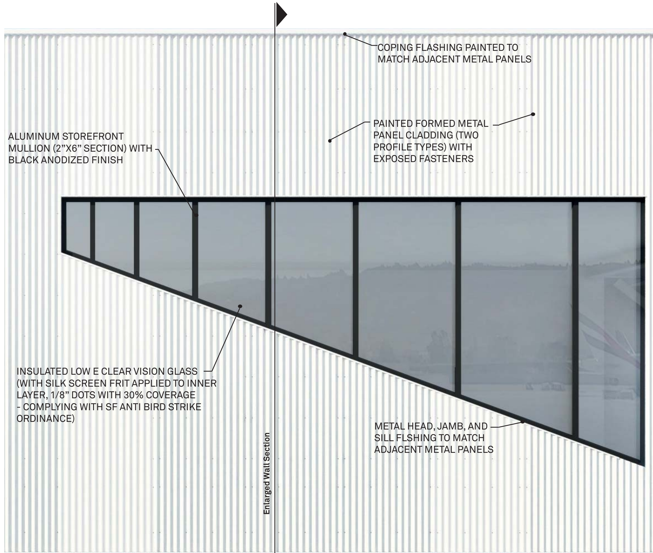
Enlarged Exterior Elevation at New Connector Bridge nts
