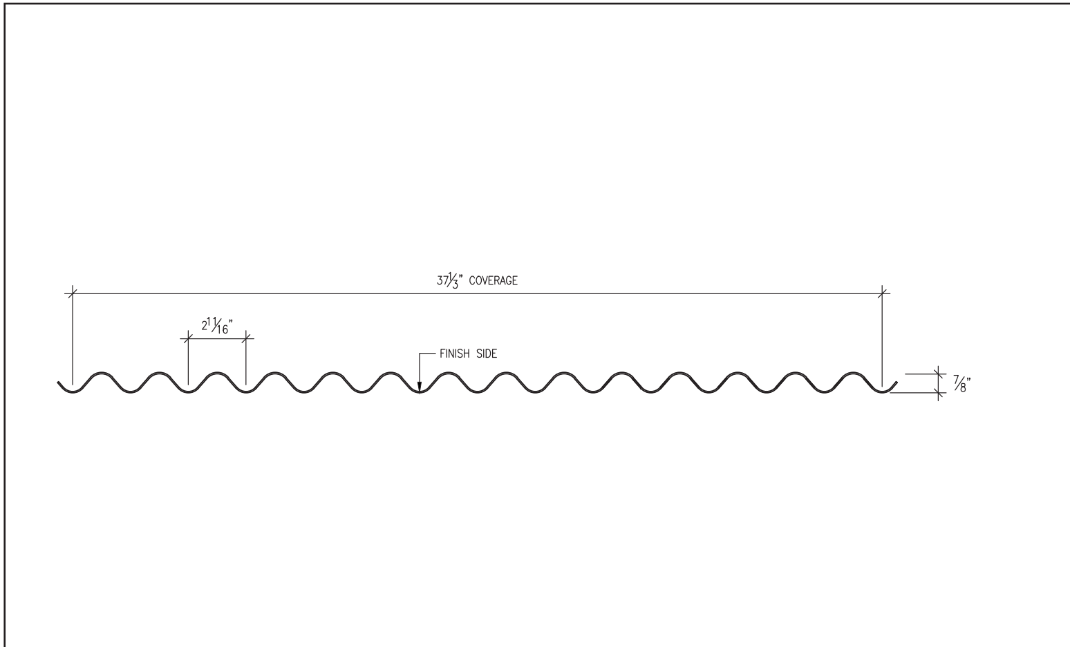
Profile Section of Formed Metal Panel - Pattern A nts
