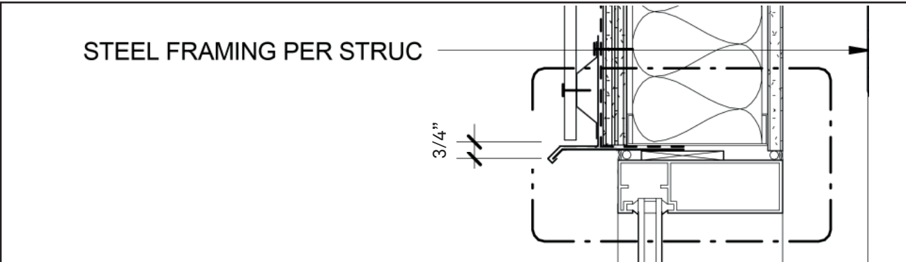
Enlarged Detail B at Exterior Window Head nts
