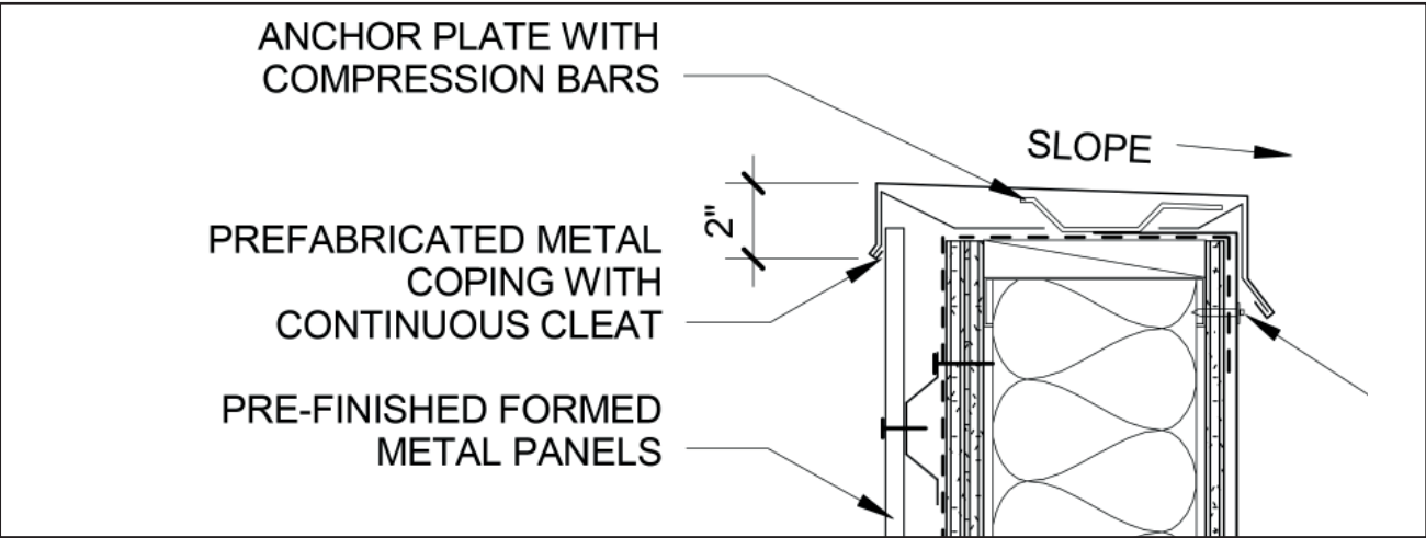
Enlarged Detail A at Exterior Wall Parapet nts
