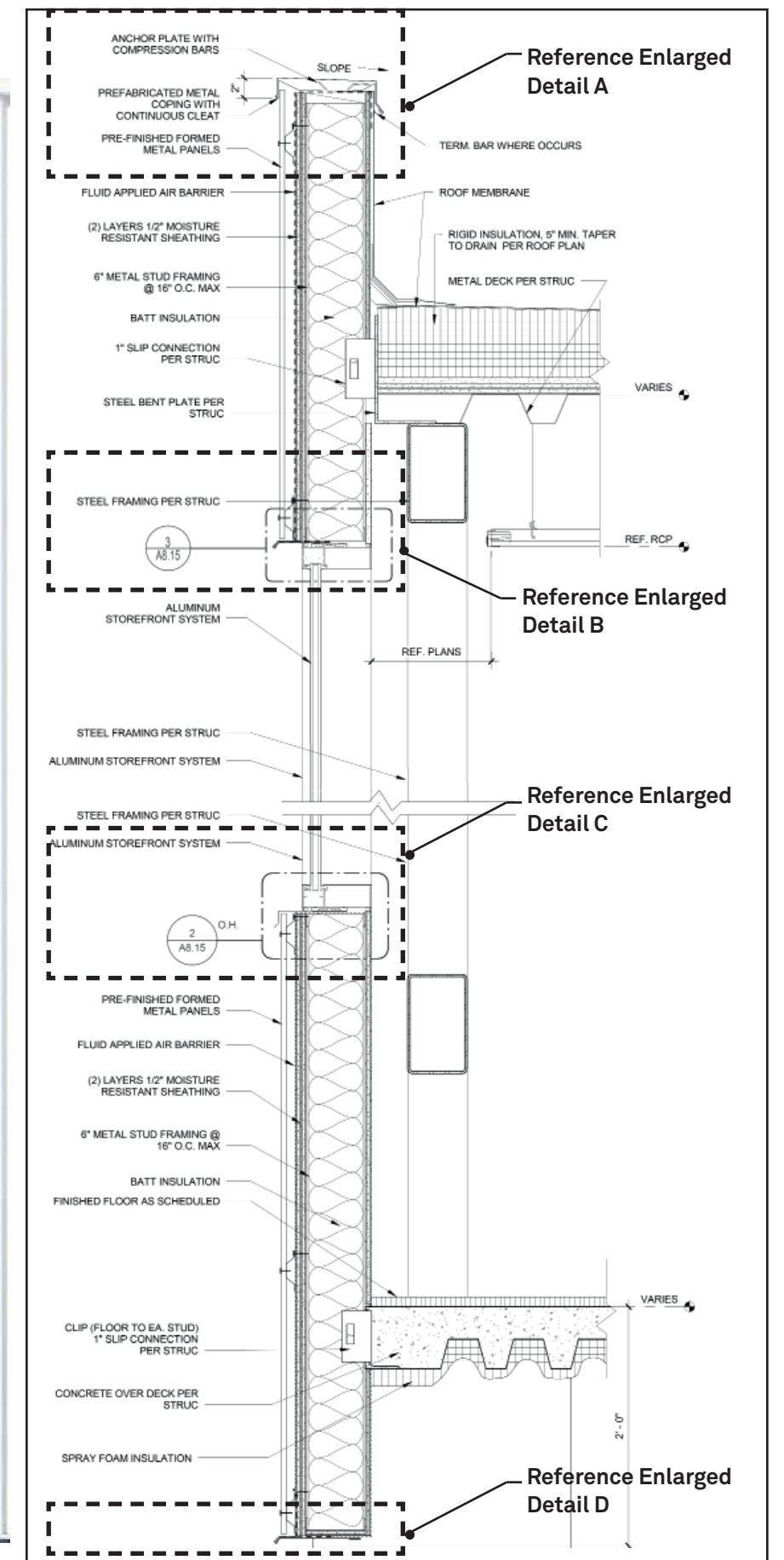
Enlarged Exterior Wall Section at New Connector Bridge nts
