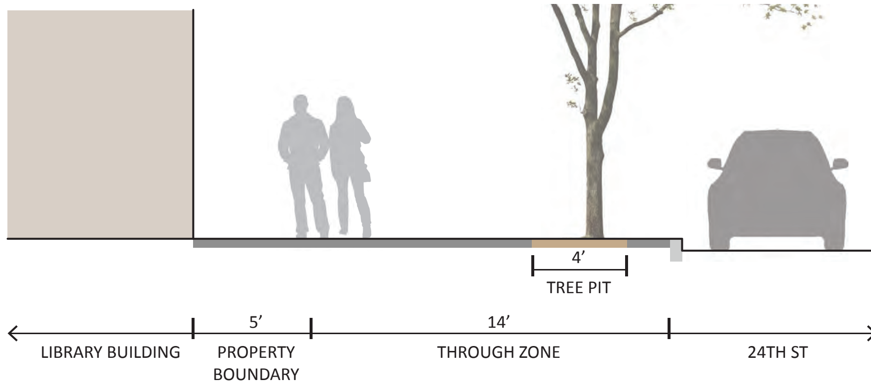
SECTION A - EXISTING CONDITION
