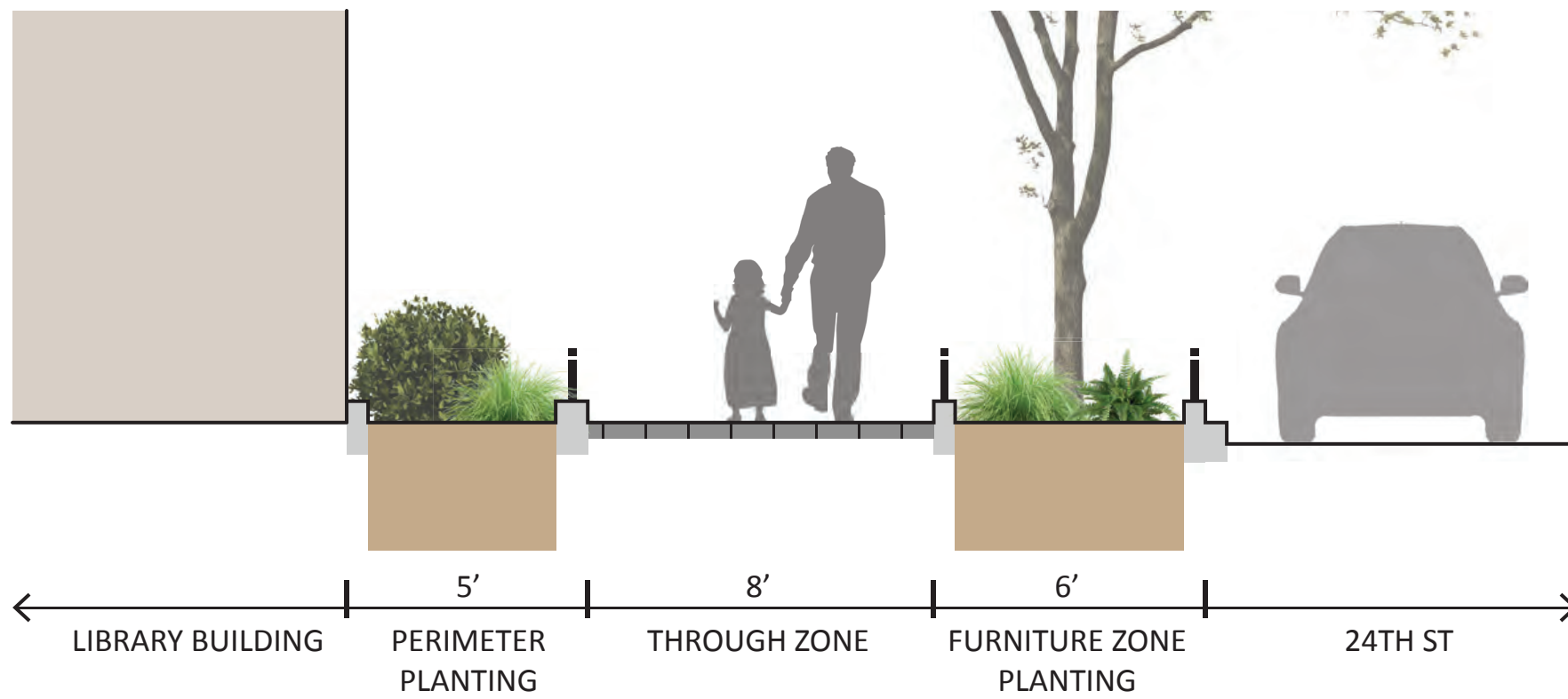
SECTION A - PROPOSED CONDITION
