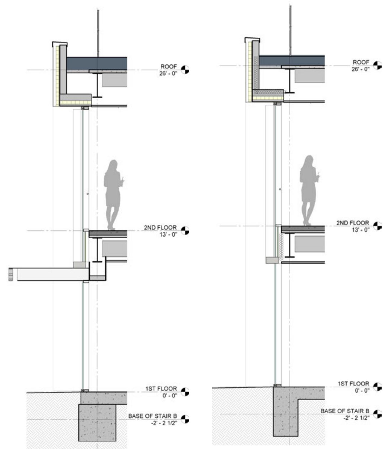
WALL SECTION A-A
