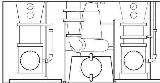
SOLIDS PRETREATMENT
