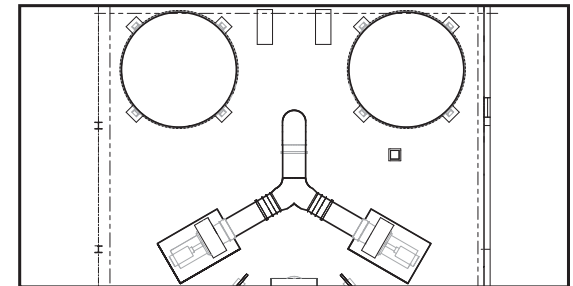
BIOSOLIDS DEWATERING
