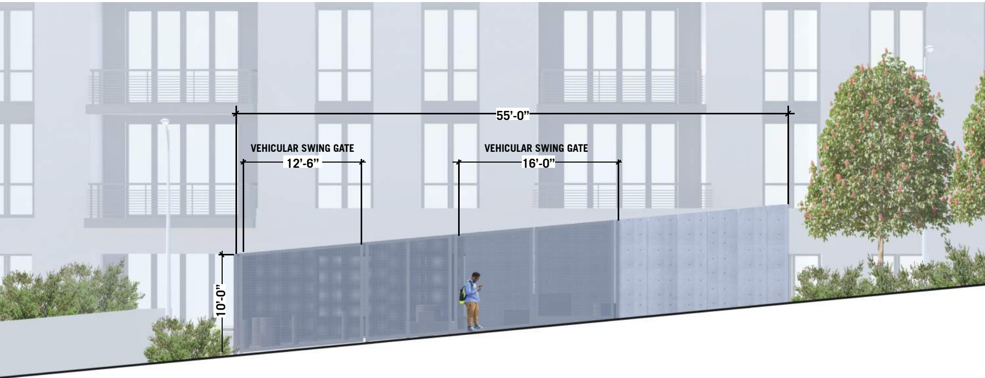
NORTH ELEVATION
