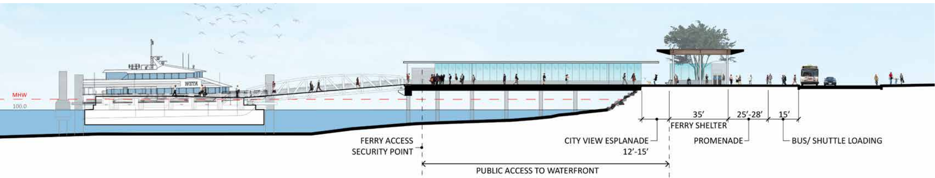
FERRY SHELTER AND PIER DETAILED SECTION
