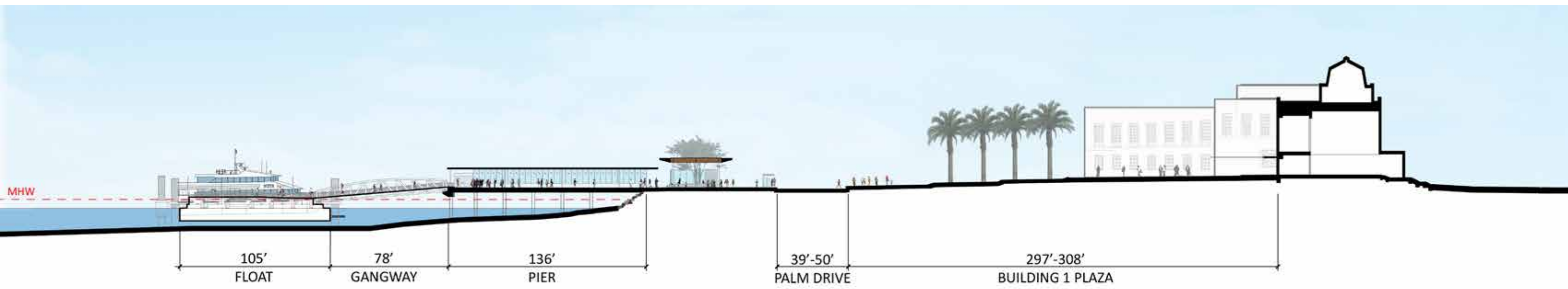
FERRY SHELTER SITE SECTION
