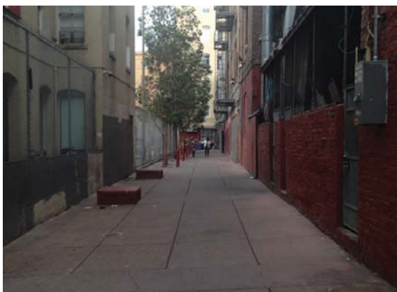
ALLEY GRADING AND LIGHTING
